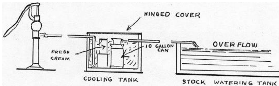
Fig. 10-Cream cooling tank arrangement showing overflow water pipe connected with stock watering tank.
