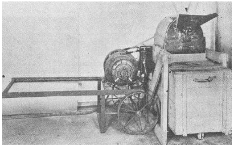
Fig. No.1. Whole grain from overhead storage conveyed to hammer mill by gravity. Ground grain drops into feed truck. Five H. P. portable motor can be used on other jobs.
